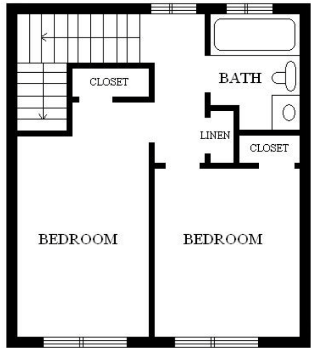
Upstairs
